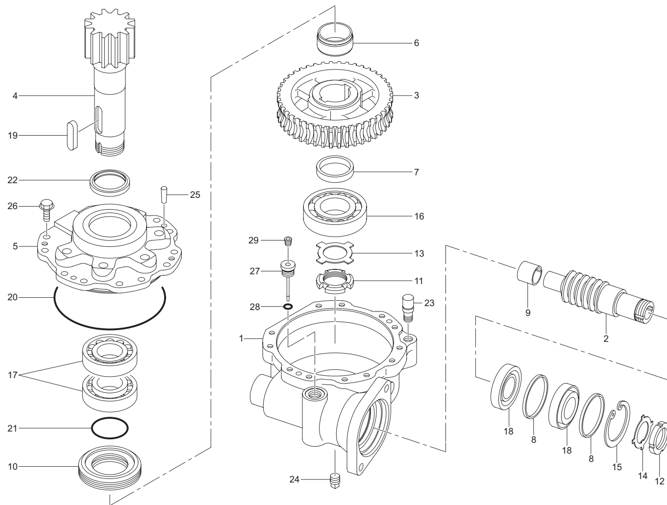
旋回減速機 ASS'Y(URV500-1-GO 系) Fig. 9-1-1 SLEWING REDUCTION GEAR ASS'Y(URV500-1-GO series)
