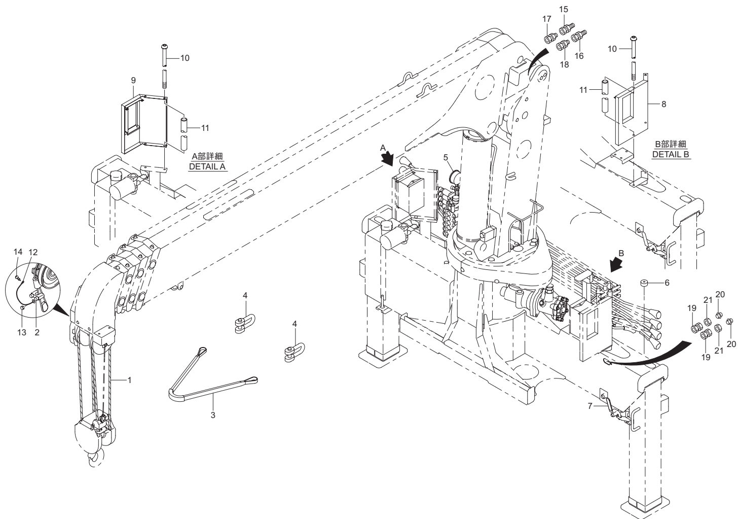
Fig. 17-2-1 装備品 (1)(URV500-1-GO 系) EQUIPMENT (1) (URV500-1-GO series)
