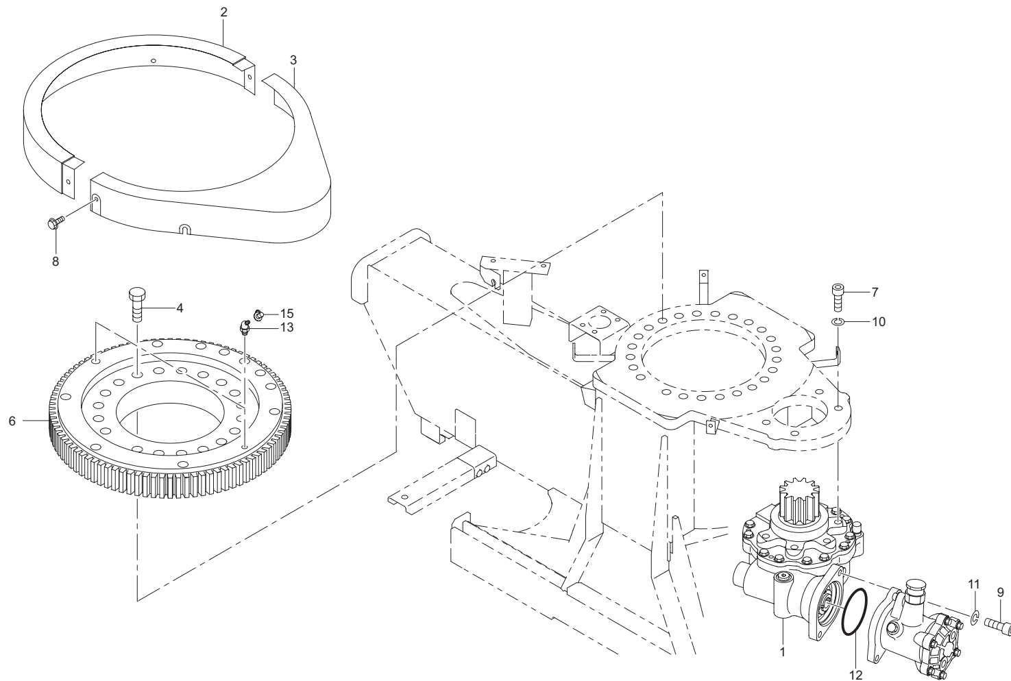
旋回装置組立 (URV500-1-GO 系) Fig. 9-1 SLEWING DEVICE ASS'Y (URV500-1-GO series)
