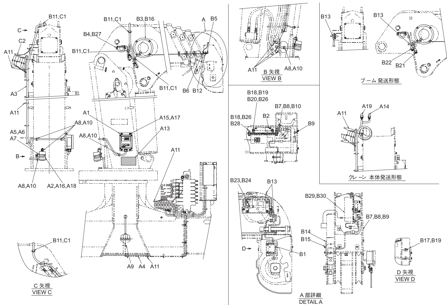
Fig. 24-8 ML FITTING WIRINGS ASS'Y (URV500-1-GO series)
