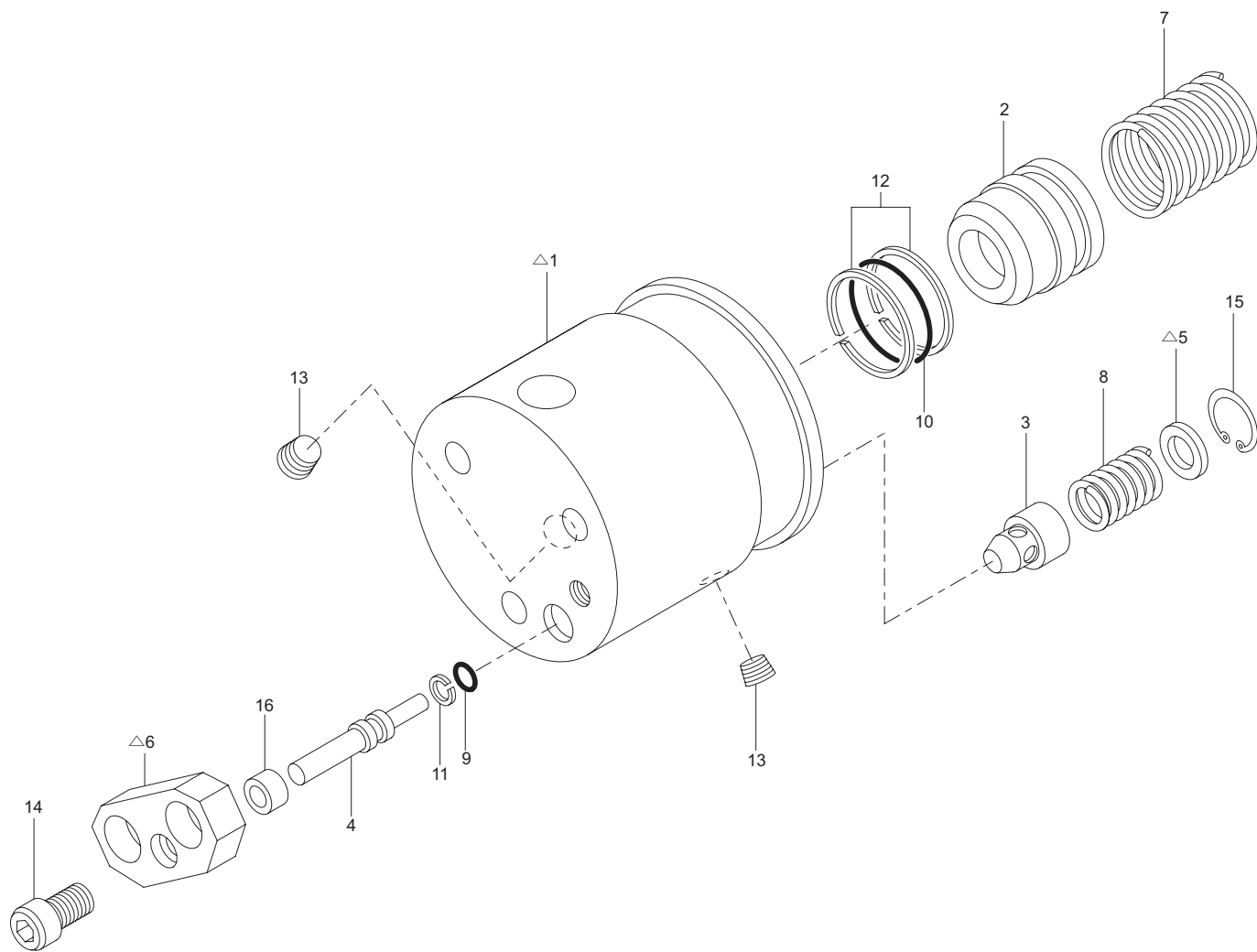
切換バルブ ASS'Y(URV503-1-G0) Fig. 2-1-1 SELECTOR VALVE ASS'Y(URV503-1-G0)
