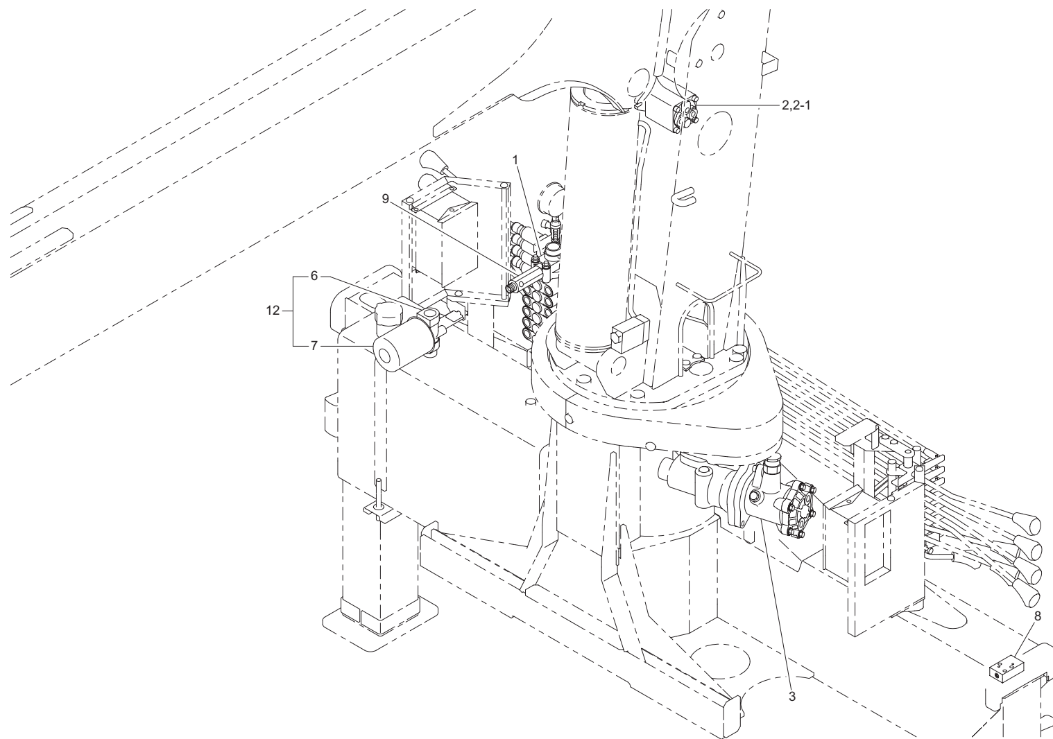
油圧駆動装置 (URV500-1-GO 系) Fig.5-2 HYDRAULIC DRIVING DEVICE(URV500-1-GO series)
