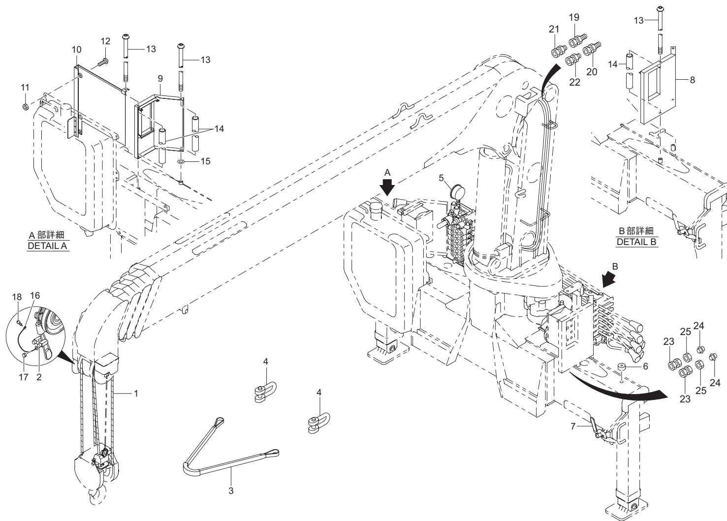
Fig. 17-2-1 装備品 (1)(URV370-GO 系) EQUIPMENT (1) (URV370-GO series)
