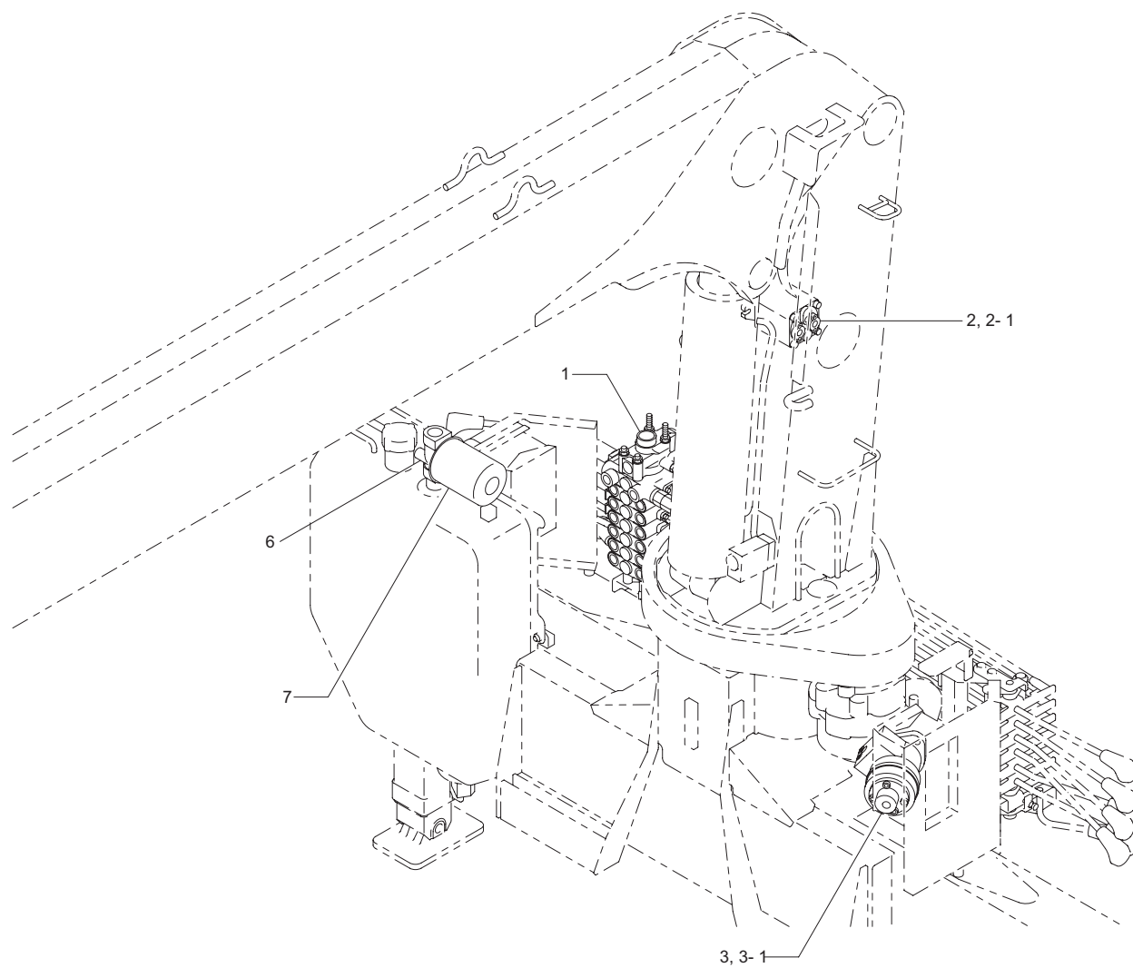
油圧駆動装置 (URV370-GO 系) Fig.5-2 HYDRAULIC DRIVING DEVICE(URV370-GO series)
