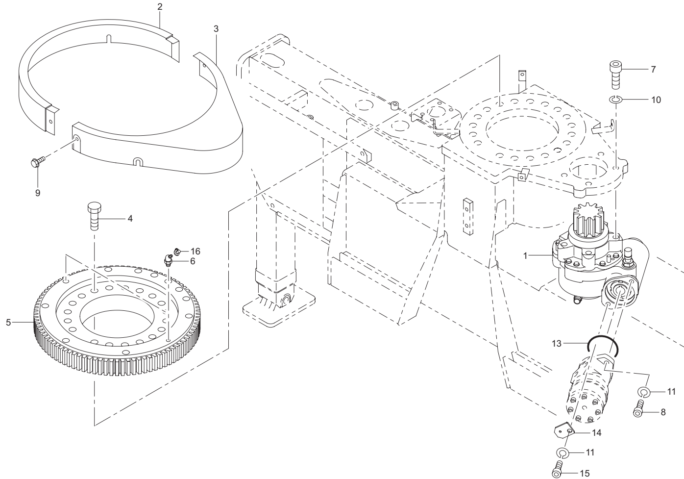
旋回装置組立 (URV370-GO 系) Fig. 9-1 SLEWING DEVICE GEAR ASS'Y (URV370-GO series)
