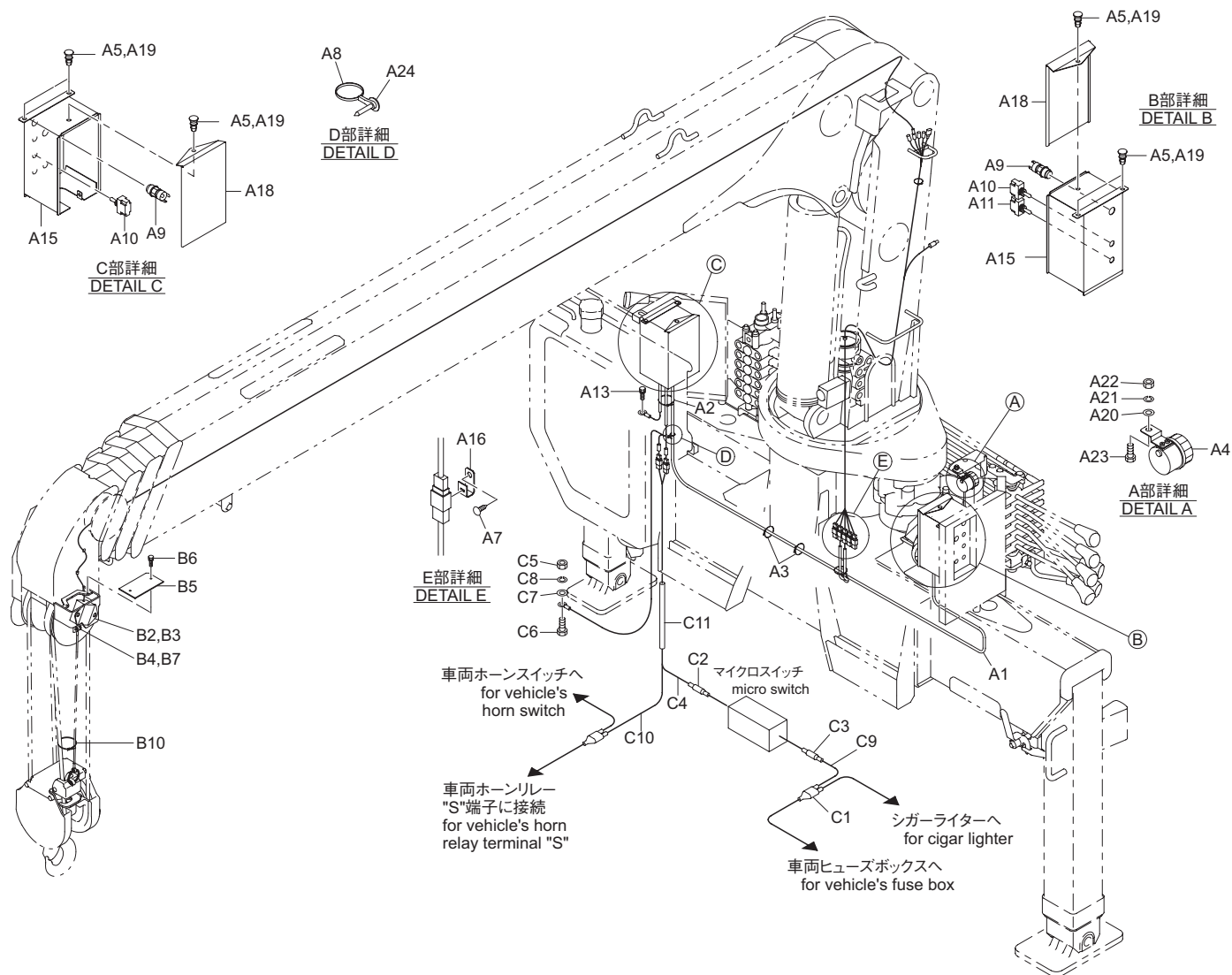
警報装置組立 (URV370-GO 系) Fig. 4-2 ALARM DEVICE ASS'Y (URV370-GO series)
