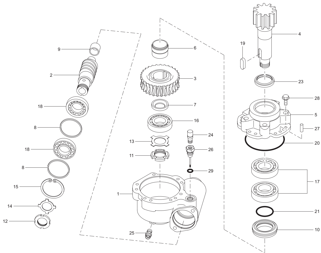
旋回減速機 ASS'Y (URV340-GO 系) Fig. 9-1-1 SLEWING DEVICE GEAR ASS'Y (URV340-GO series)
