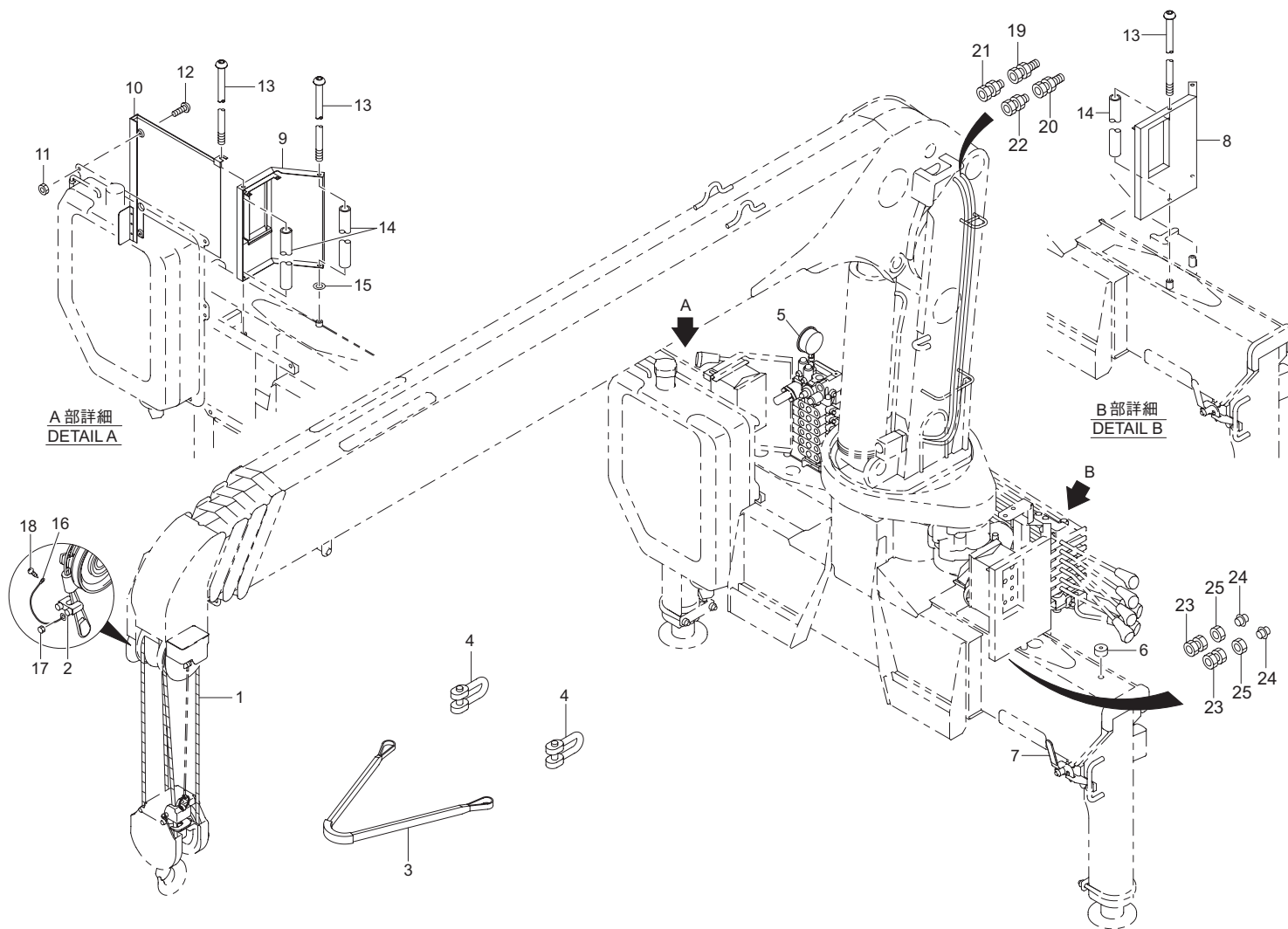
Fig. 17-2-1 装備品 (1)(URV340-GO 系) EQUIPMENT (1)(URV340-GO series)
