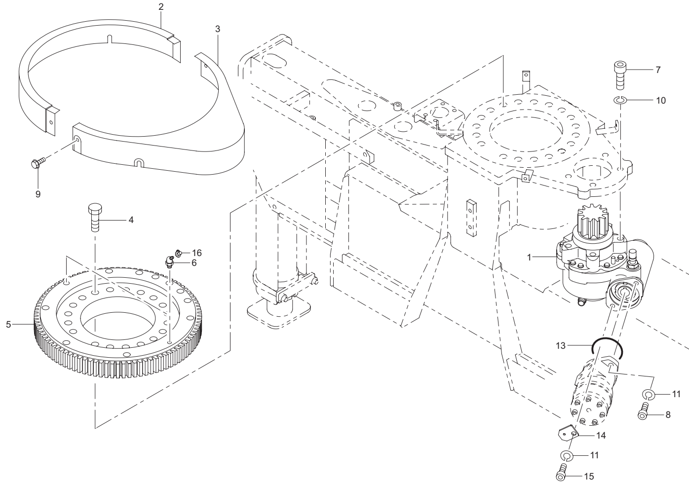
旋回装置組立 (URV340-GO 系) Fig. 9-1 SLEWING DEVICE GEAR ASS'Y (URV340-GO series)
