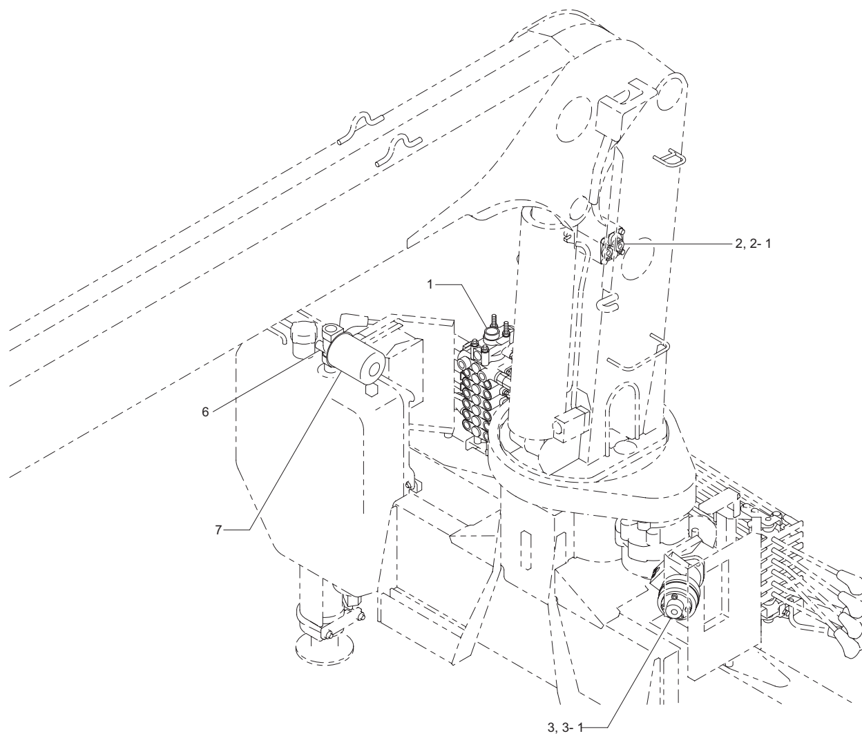
油圧駆動装置 (URV340-GO 系) Fig.5-2 HYDRAULIC DRIVING DEVICE(URV340-GO series)
